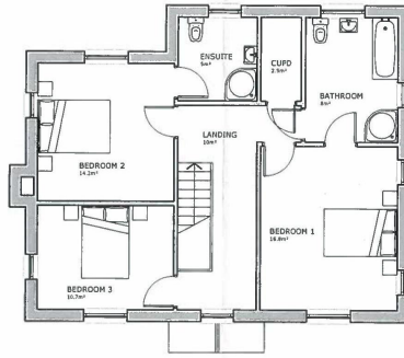
02 PROPOSED FIRST FLOOR PLAN 1:100
