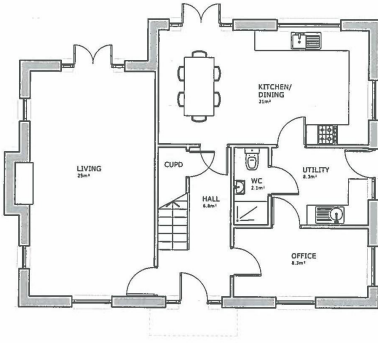
01 PROPOSED GROUND FLOOR PLAN 1:100
